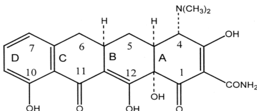
Figure.n°09: Structure de la 6-deoxy-6-demethyltétracycline (the minimum tetracycline pharmacophore) (mabr.asm.org).
