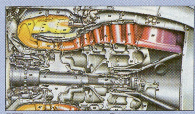
PW545 cutaway poster - P41
