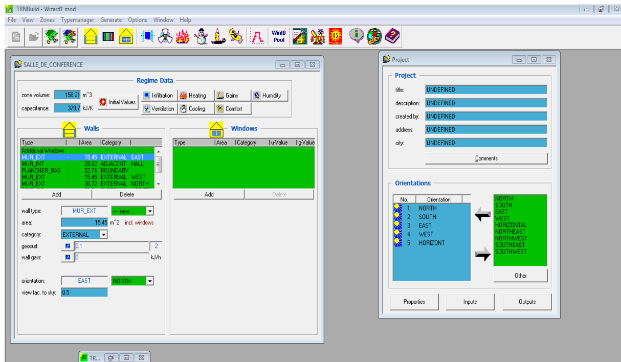
Figure 47 Interface TRNBUILD.
