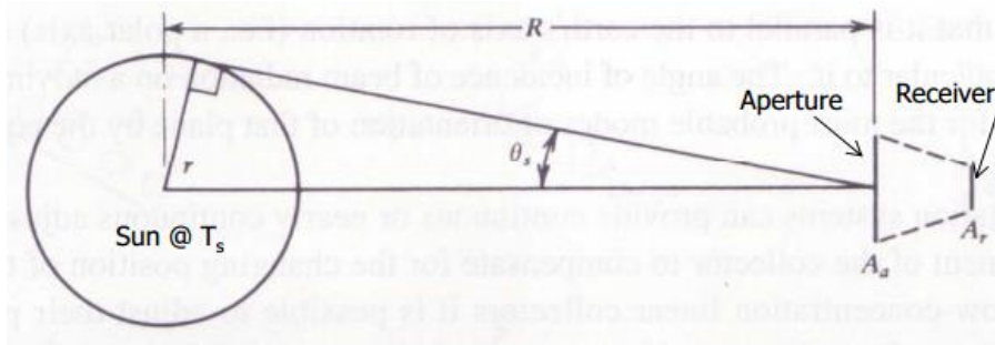
Figure 17: concentrating ratio schematic
