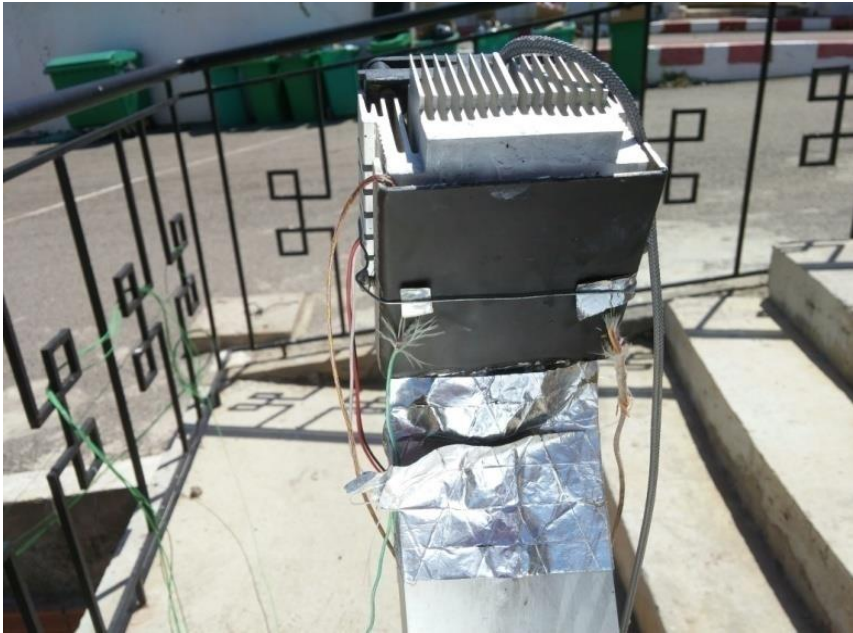
Figure 32: The assembled heat transfer system
