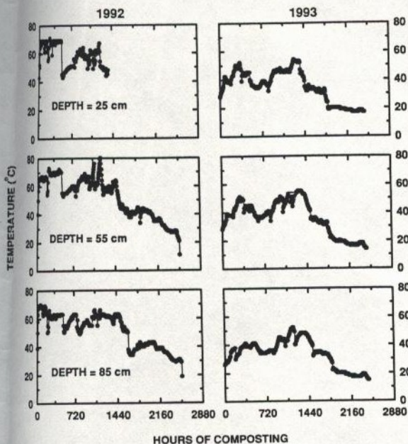
Fig. 1. Temperature of the feedlot manure composting windrows at three depths in 2 yr at Mead, NE.
