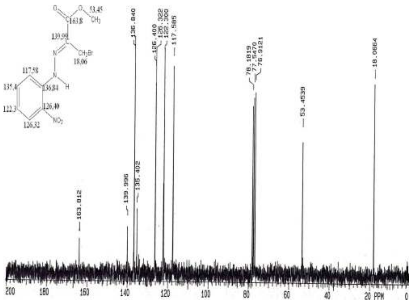
Figure 16 : Spectre 13 C-RMN de (E)-3-bromo-2- (2'-nitrophenyl)hydrazono propanoate de méthyle.
