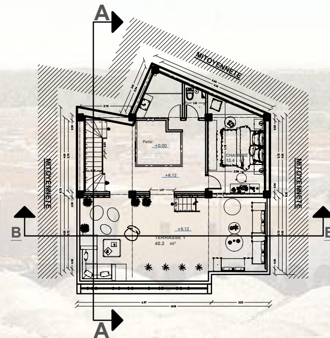
PLAN 2 EME ETAGE
