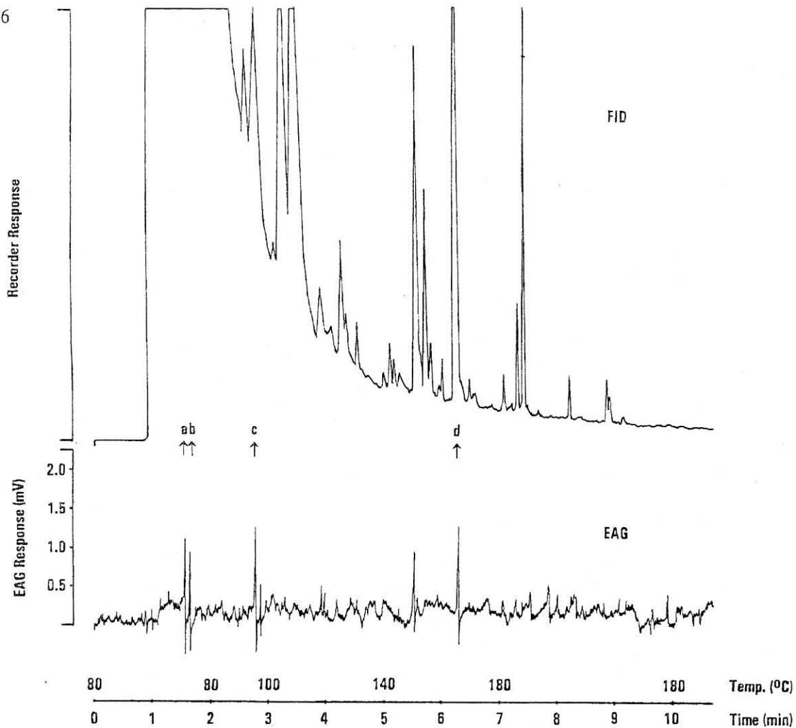
Fig. 1. Simultaneously recorded gas chromatogram (FID) of trapped volatile compounds from fungus-infected date fruits, Phoenix dactylifera , on a DB-225 capillary column, and electroantennogram (EAG) from a female carob moth, Ectomyelois ceratoniae . Retention times of synthetic standards acetaldehyde (a), ethanol (b), ethyl hexanoate (c), and 2-phenylethanol (d) are indicated.
