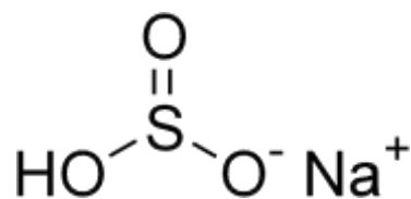
Figure 25: Structure de bisulfite de sodium (82)
