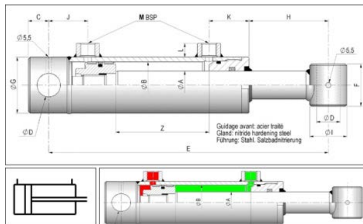
Figure 3.17: Vérin hydraulique double effet.
