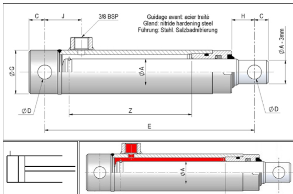
Figure 3.16: Vérin hydraulique simple effet.
