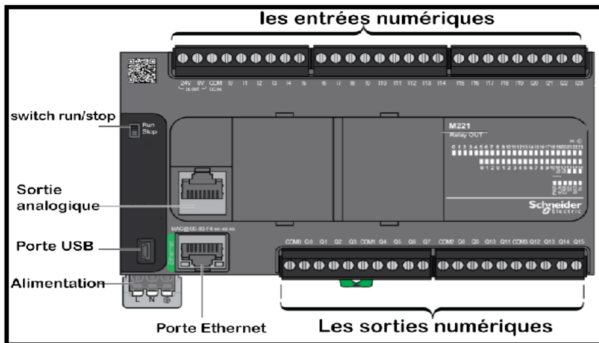
Figure3.11: L'automate programmable industriel Schneider Electric TM221CE40R.
