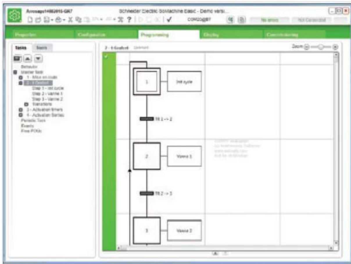
Figure 3.6: Langage graphique GRAFCET.
