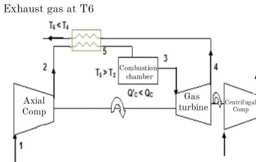
Figure3.24: Turbine cycle with a heat recovery system.
