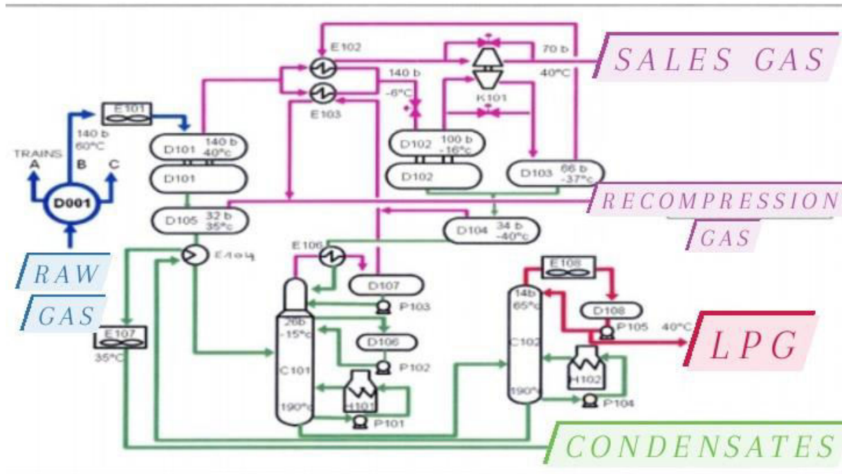
Figure1.5. HUDSON process [2]
