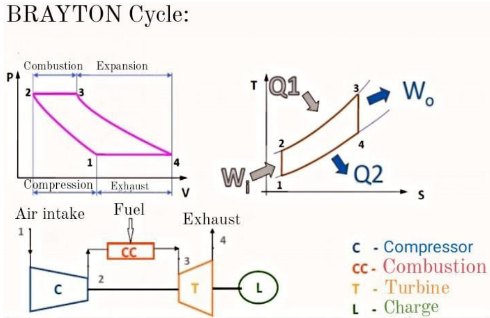
Figure.3.2 Theoretical cycle of BRAYTON (Temperature - Entropy. S) [6]
