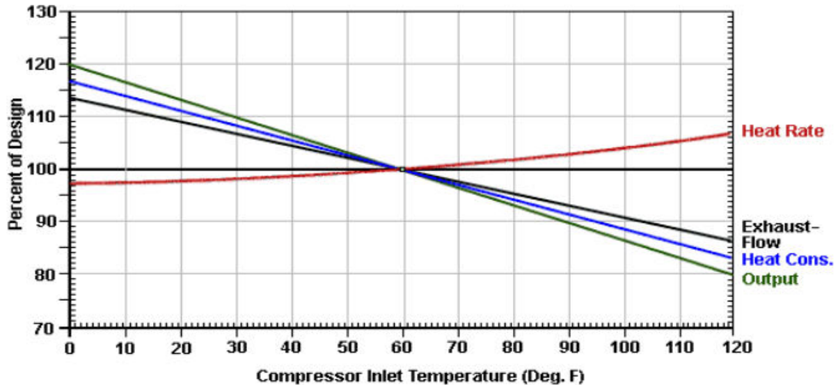
Figure.3.21 Influence of ambient temperature on the performance of GE gas turbines
