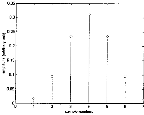
Figure 7.5. The filter h(n) .
