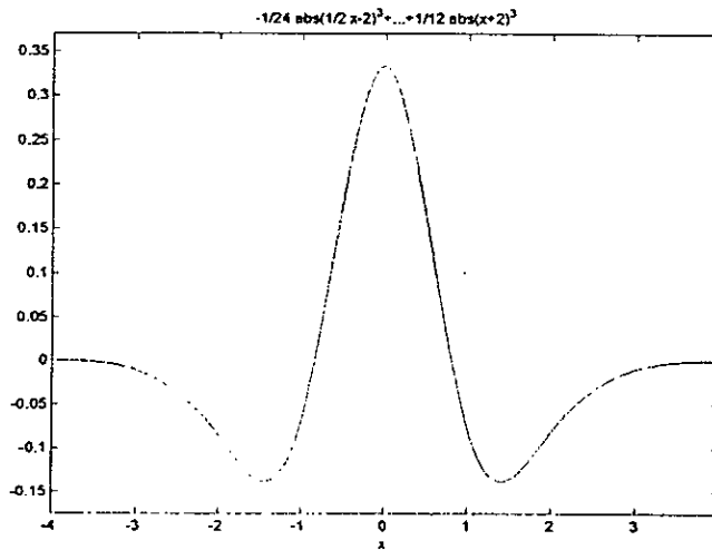
Figure III-19. The wavelet \psi .
