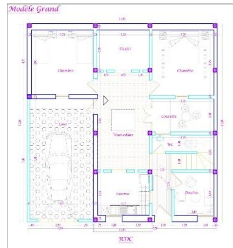
Figure 132: plan RDC du type grand. Source: fondation amidoul
