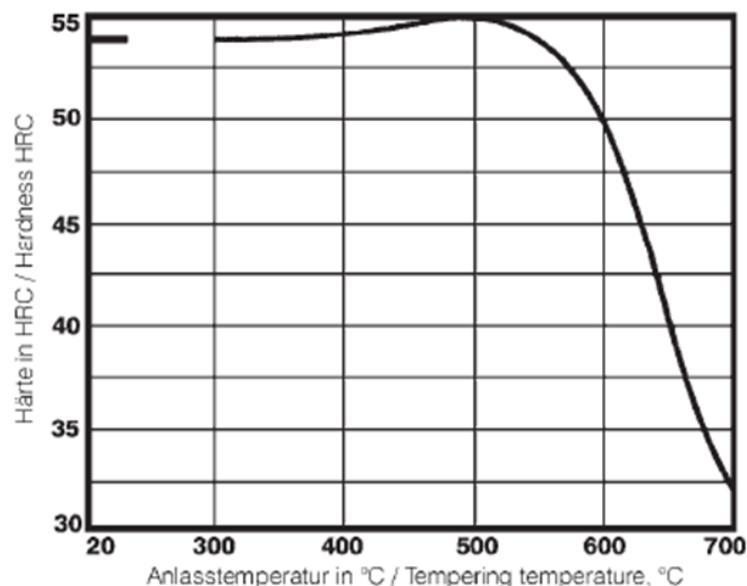
Figure 2.6 Courbe de temperature HRC.[22]
