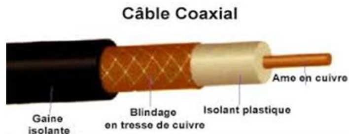
Figure.I.6 : Câbles coaxial
