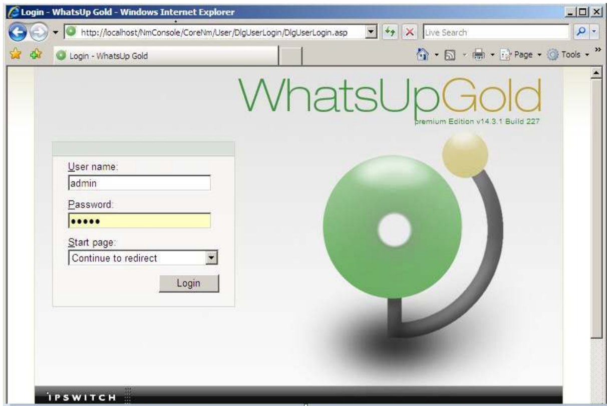
Figure IV.2 : l' Authentification.
