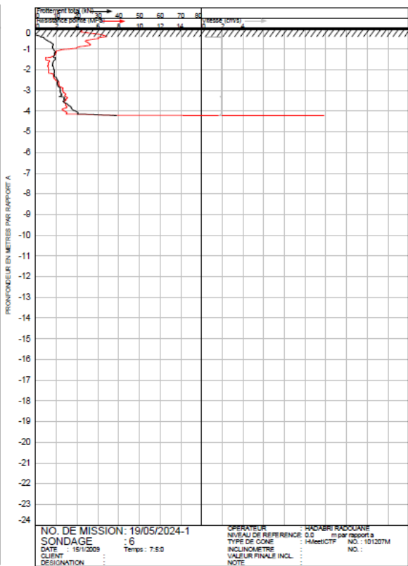
Figure 3.26 : PK 41+470 CPT06-02
