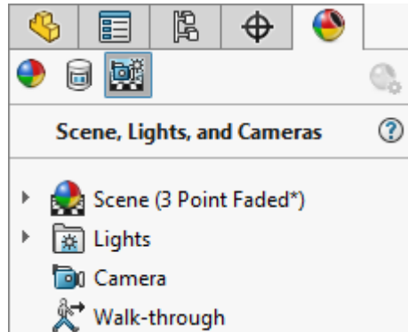
Fig.4.5: Display Manager [20]
