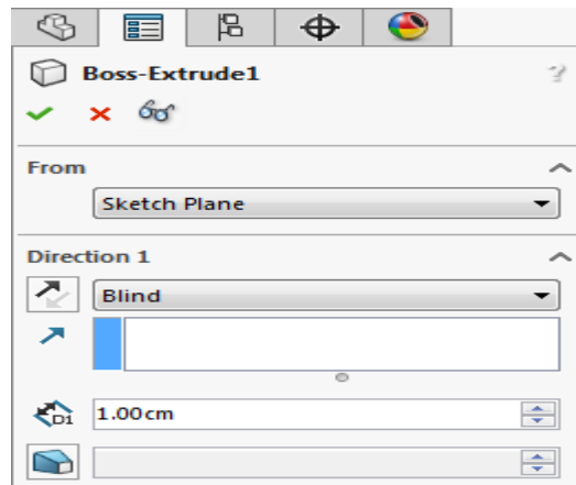
Fig.4.2: Property Manager [20]
