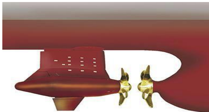
Fig.1.7: Hélices contrarotatives. [15]
