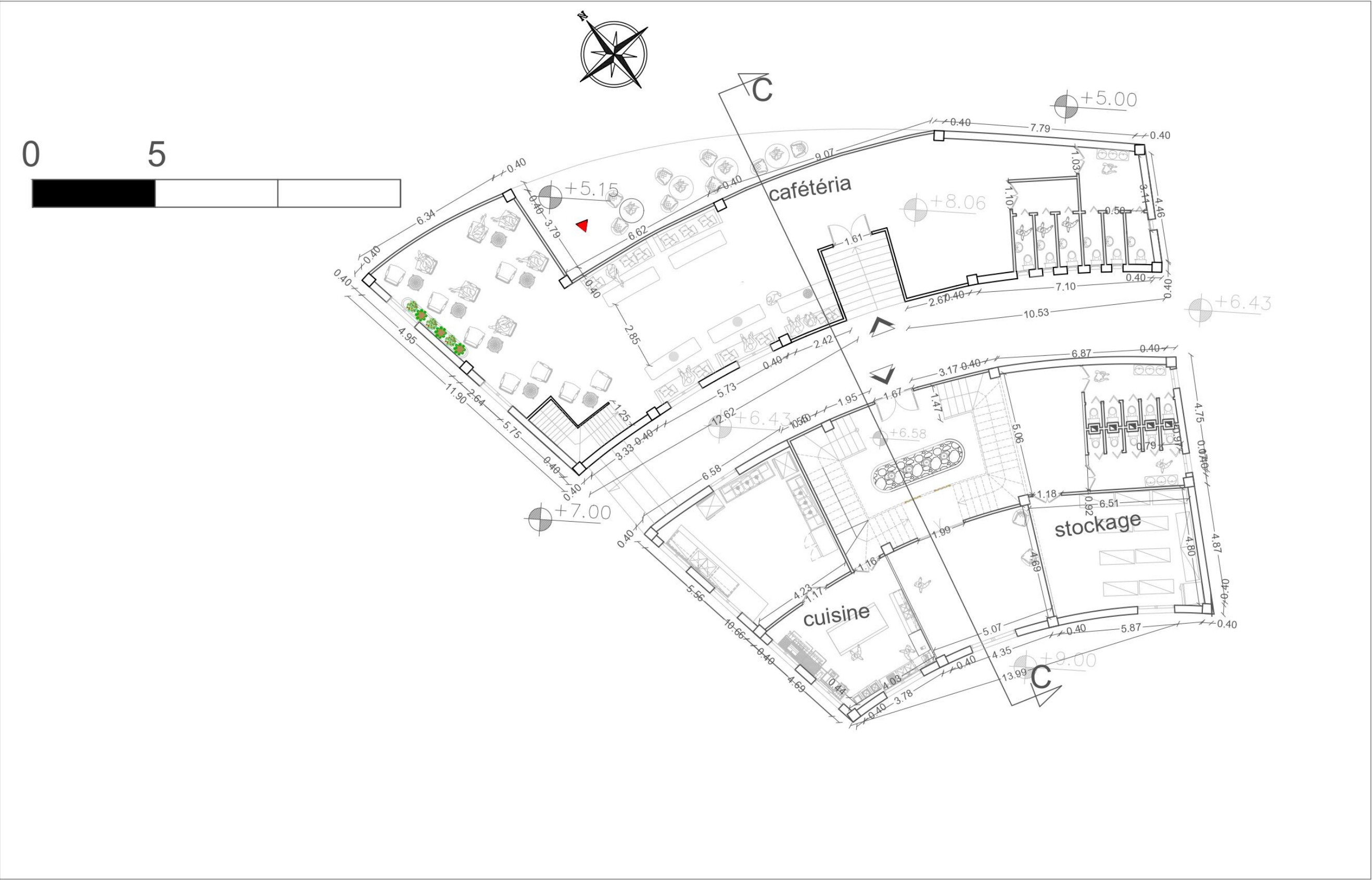
SOCLE : R+1 CAFETERIA / REZ-DE-CHAUSSEE RESTAURANT
