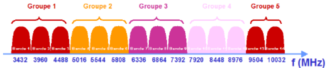
Figure 1.11 : OFDM Multi-Bandes
