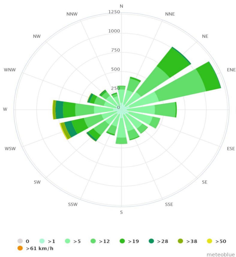
Figure 2.rose des vents
