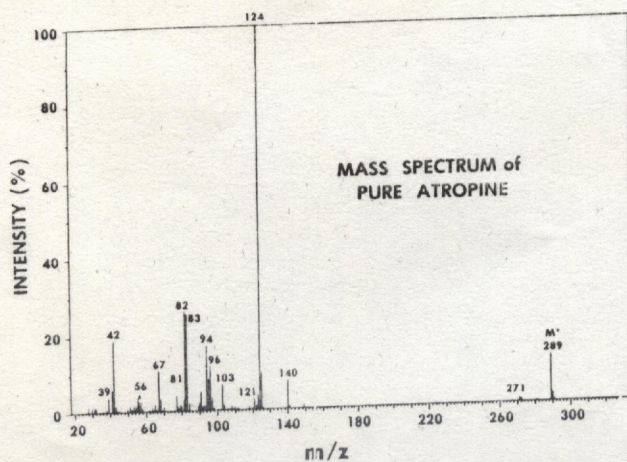
Figure 1. Mass spectrum of atropine.
