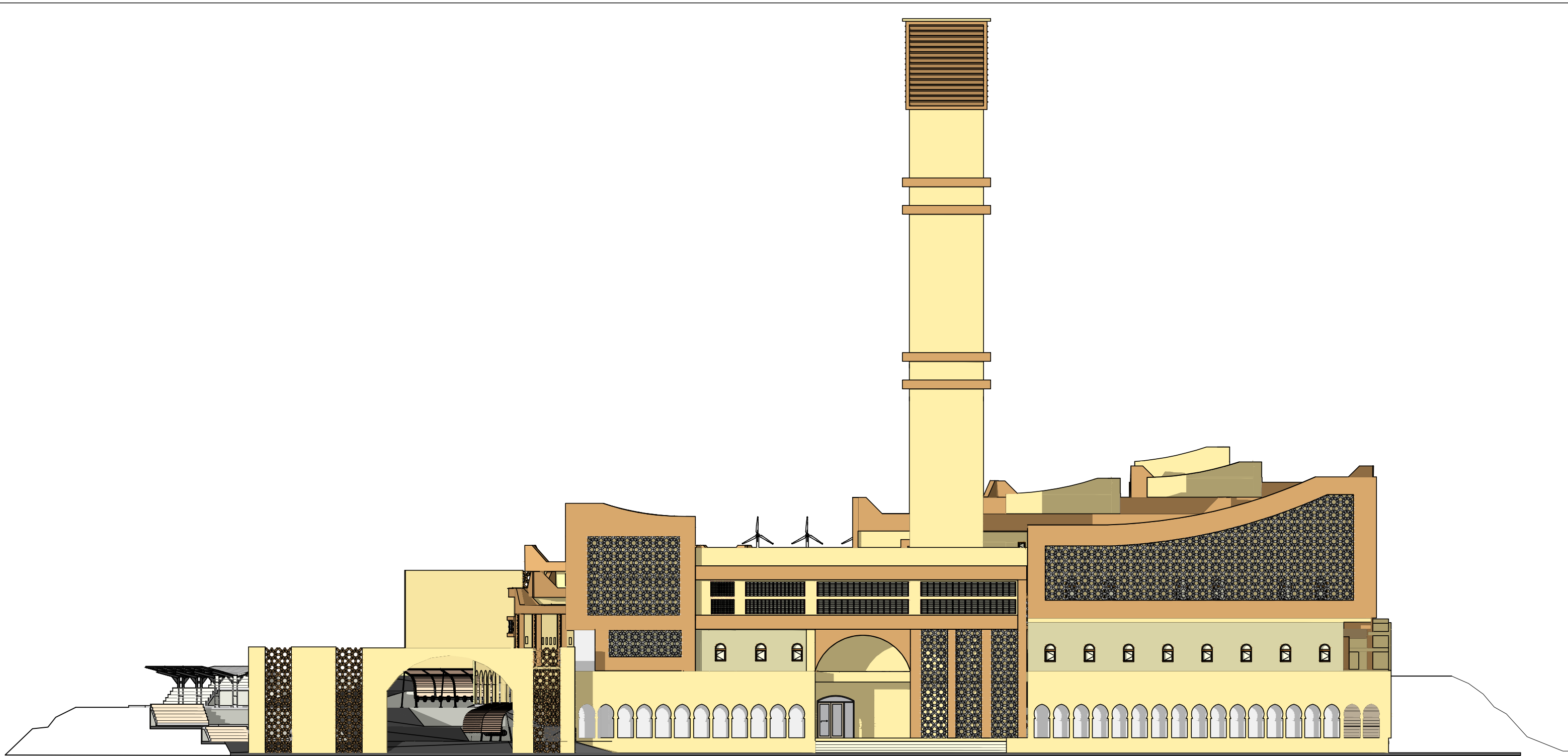
Façade principale
