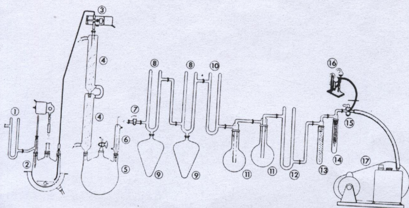
Fig. 5. An apparatus for the isolation of volatiles from solid or aqueous foods by evaporation from a continuous thin heated film under vacuum.
