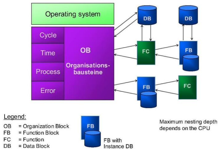
Figure II.4 : Blocs de programmation
