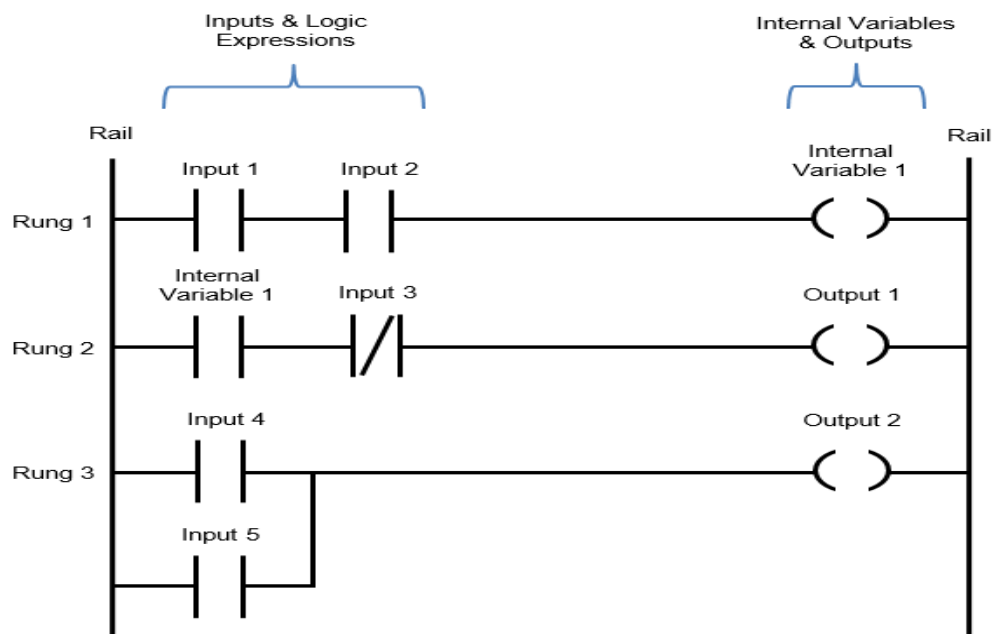
Figure III.4: Langage LADDER
