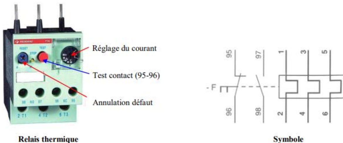
Figure II.17 : Relais thermique
