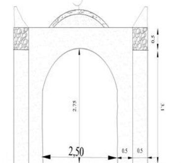
Section C-C deC1 ech:1/50
