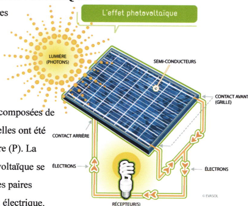
Figure n°=28 la conversion photovoltaïque
