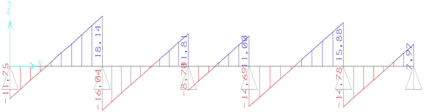
Figure III.18 Efforts Tranchants ELU
