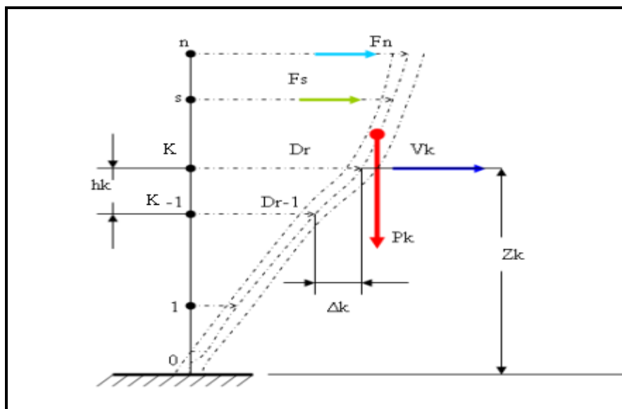
Figure : Effet P-delta
