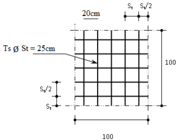
Figure III.19 : Ferrailage de la dalle de compression
