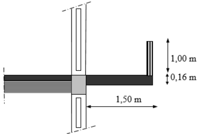
Figure III-5 Dimension du balcon
