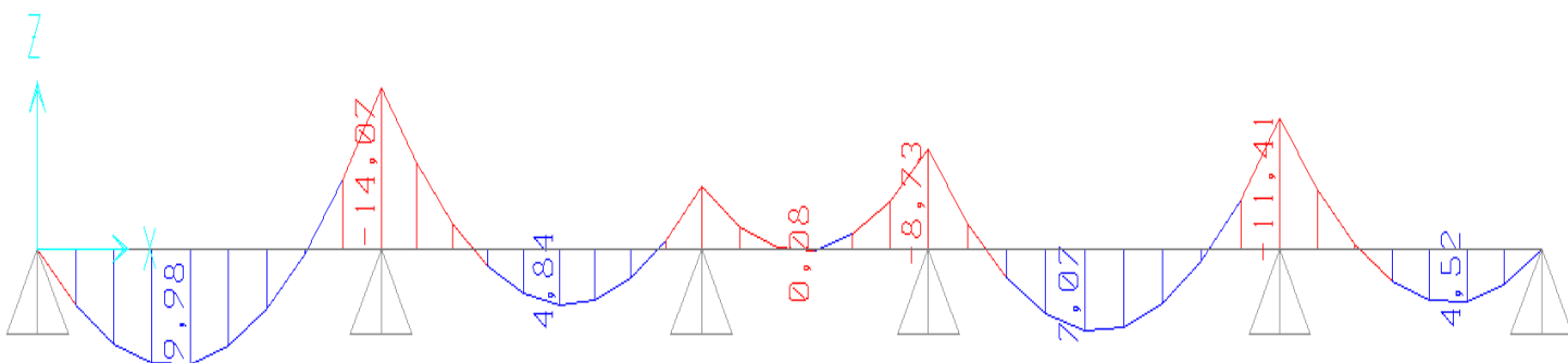
Figure III.17 Moments ELU
