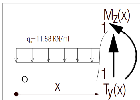
Figure III-10 – Tronçon (1-1)
