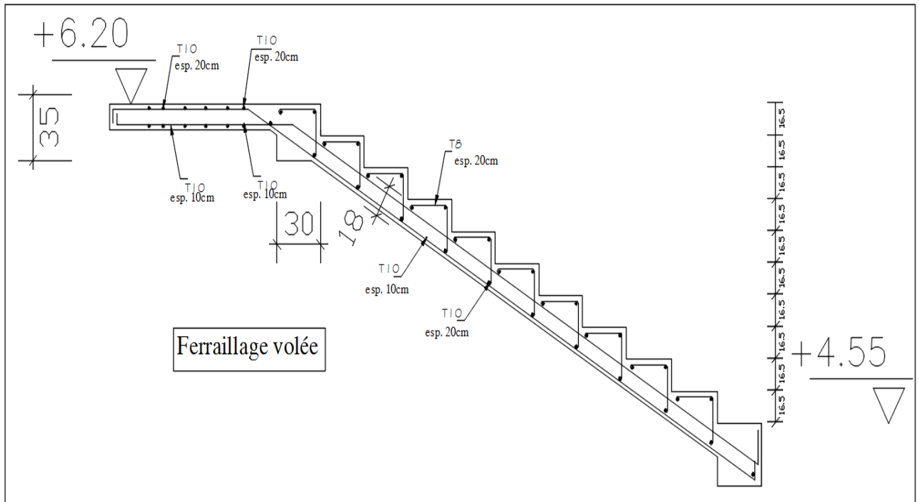
Figure III.14 : Ferrailage escalier
