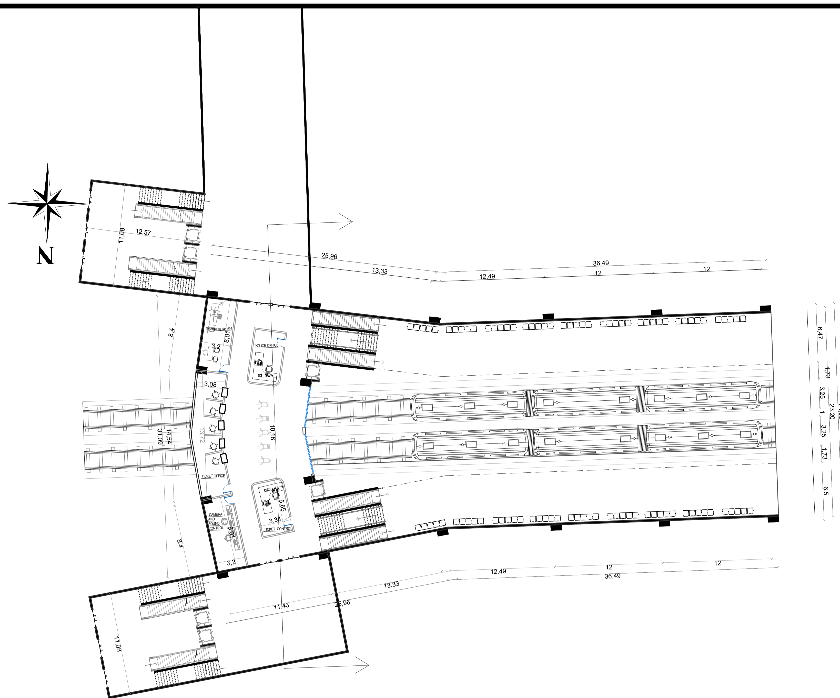
UNDER GROUND FLOOR PLAN -3,8m
