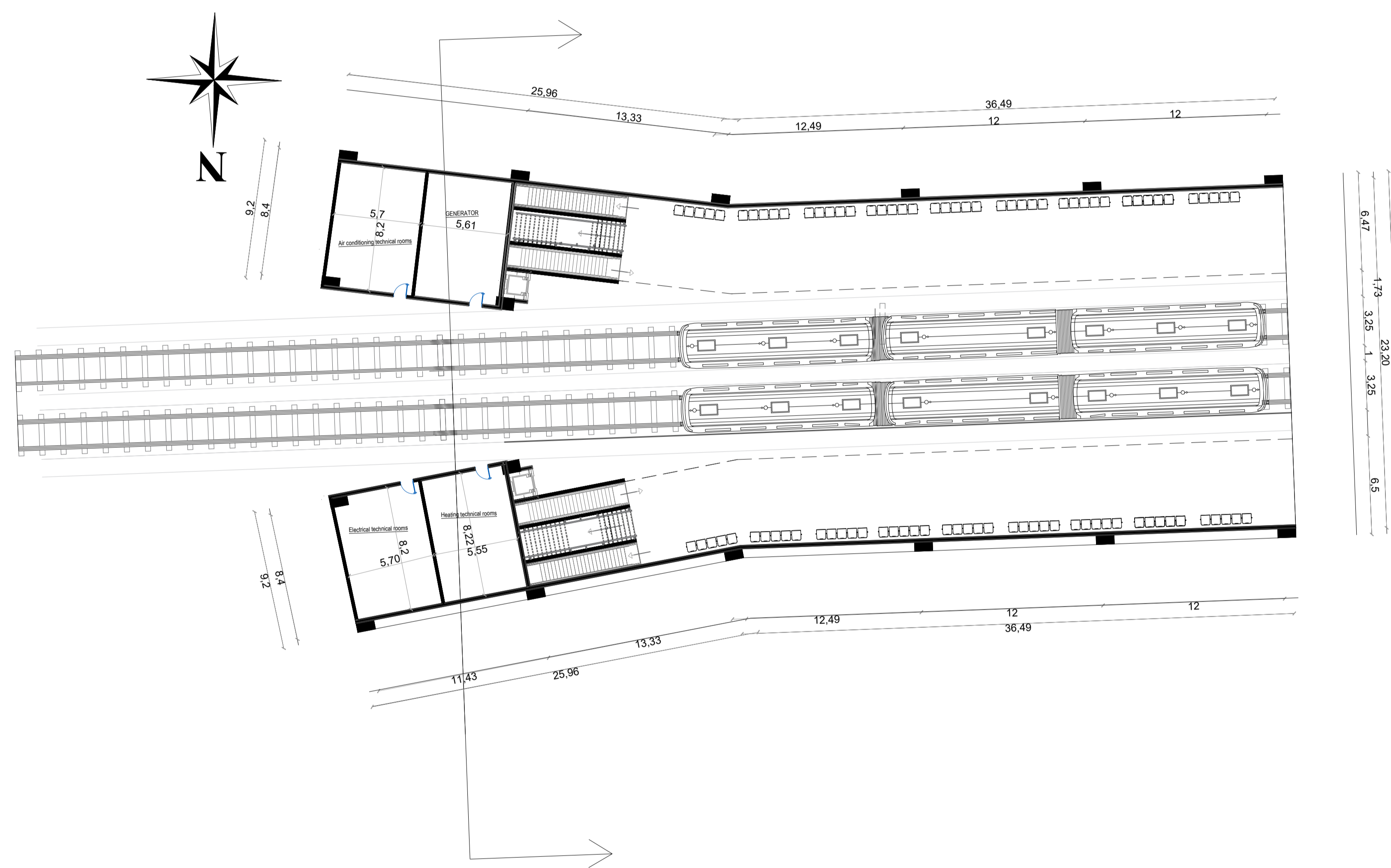
UNDER GROUND FLOOR PLAN -10m
