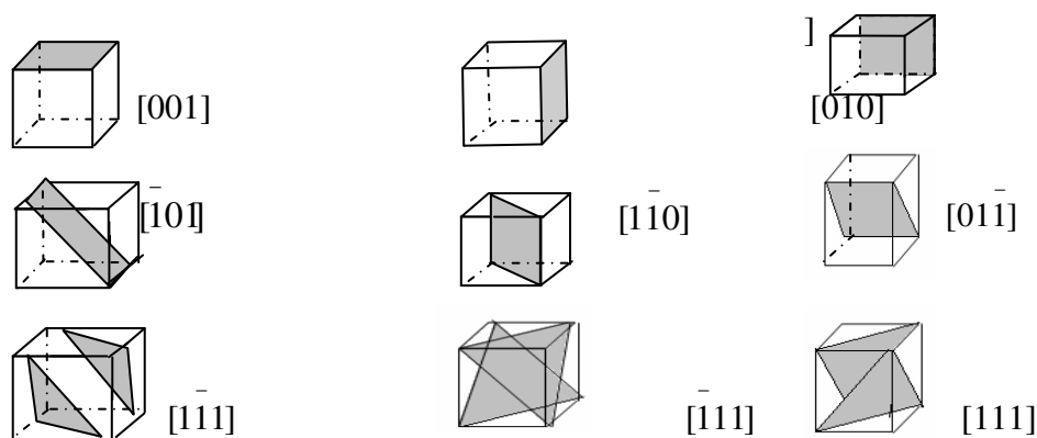
Figure I-2 Plans de structures cubiques
