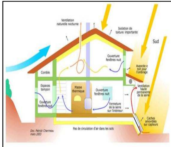
Figure 1-4-1architecture bioclimatique
